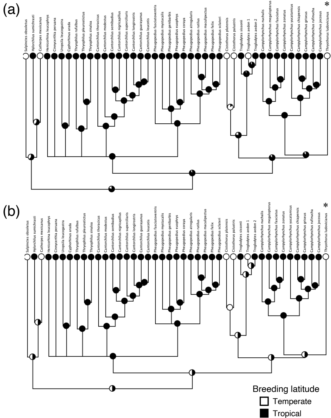
FIGURE S3. Ancestral character state reconstructions of breeding latitude on a phylogeny of 42 wren species, with black and white fill showing (a) proportional likelihoods from Markov k-state one parameter maximum-likelihood analysis or (b) character states resolved using unordered parsimony. Carolina wren ( Thyrothorus ludovicianus ) is indicated by an asterisk.
