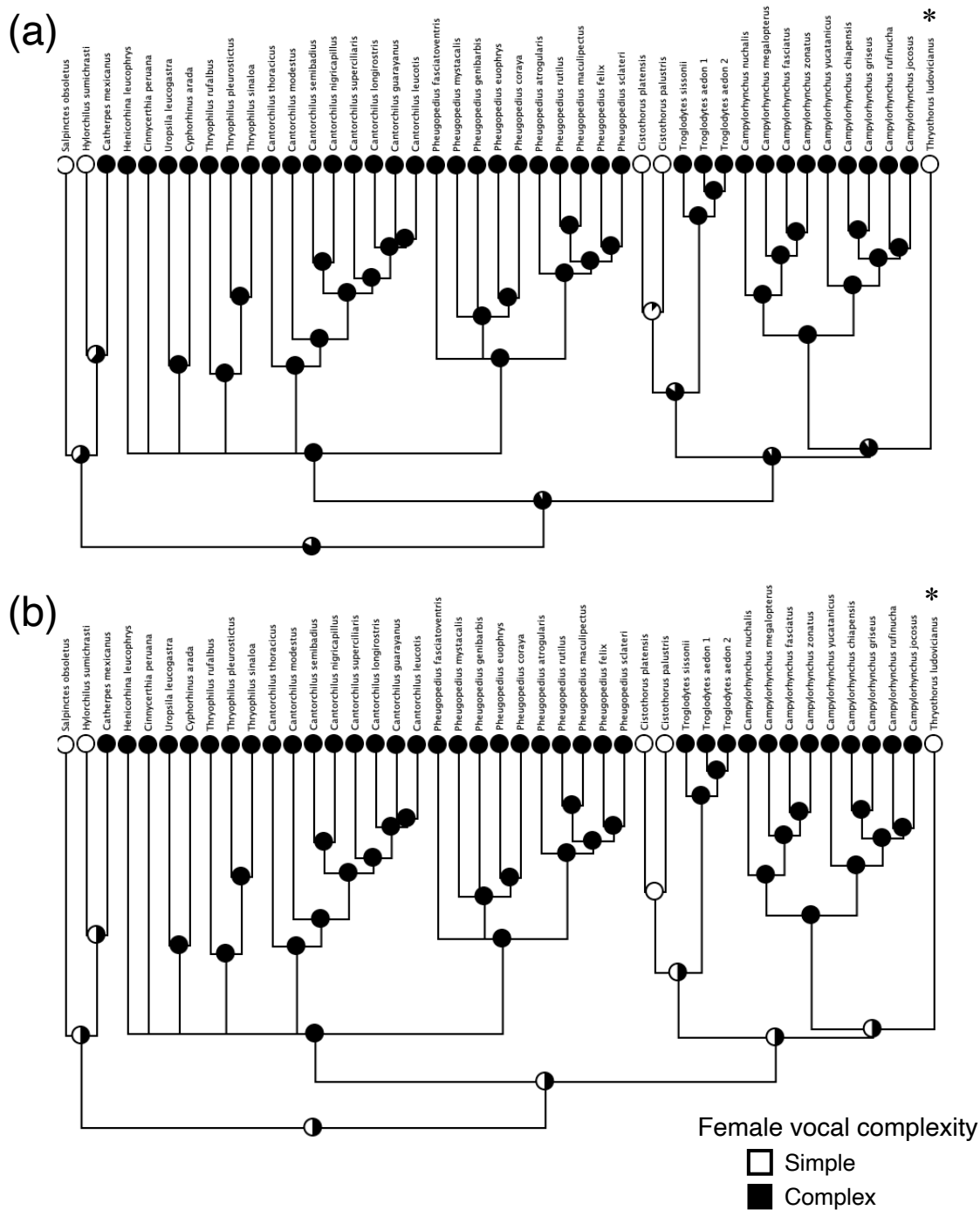
FIGURE S1. Ancestral character state reconstructions of female vocal complexity on a phylogeny of 42 wren species, with black and white fill showing (a) proportional likelihoods from Markov k-state one parameter maximum-likelihood analysis or (b) character states resolved using unordered parsimony. Carolina wren ( Thyrothorus ludovicianus ) is indicated by an asterisk.
