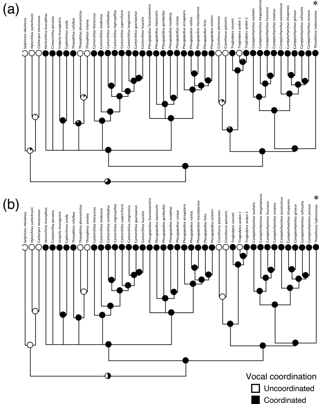
FIGURE S2. Ancestral character state reconstructions of vocal coordination between males and females on a phylogeny of 42 wren species, with black and white fill showing (a) proportional likelihoods from Markov k-state one parameter maximum-likelihood analysis or (b) character states resolved using unordered parsimony. Carolina wren ( Thyothorus ludovicianus ) is indicated by an asterisk.
